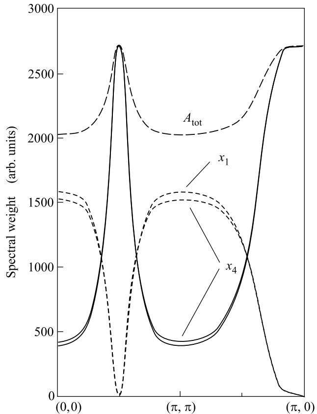
Fig.3. Partial weights of the triplet states (dotted line) and singlet states (solid line) to A_{\text{tot}} - total spectral intensity at two different Y-contents, x_1 > x_4 . Here the spectral function A(\mathbf{k}, \omega) is taken along the peak positions in the (\mathbf{k}, \omega) plane according to the dispersion shown in Fig.1
