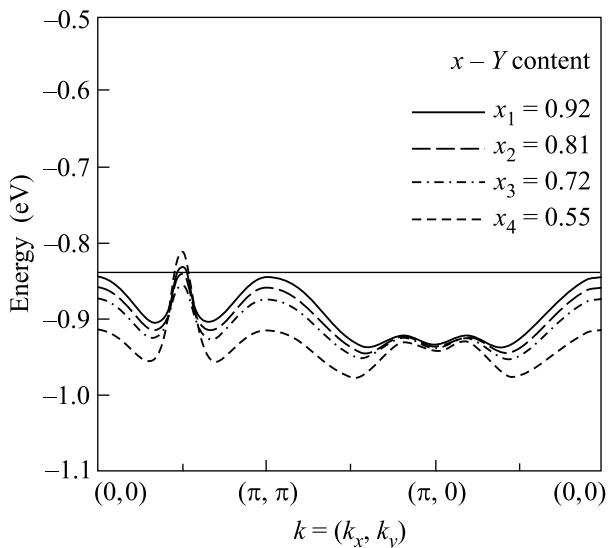
Fig.2. The dispersion of the top of the valence band calculated by the GTB method for different Y-contents x . Y( x ) as indicated in the figure. The respective t_{pp} and t'_{pp} hopping parameters used for the calculations are given in table
